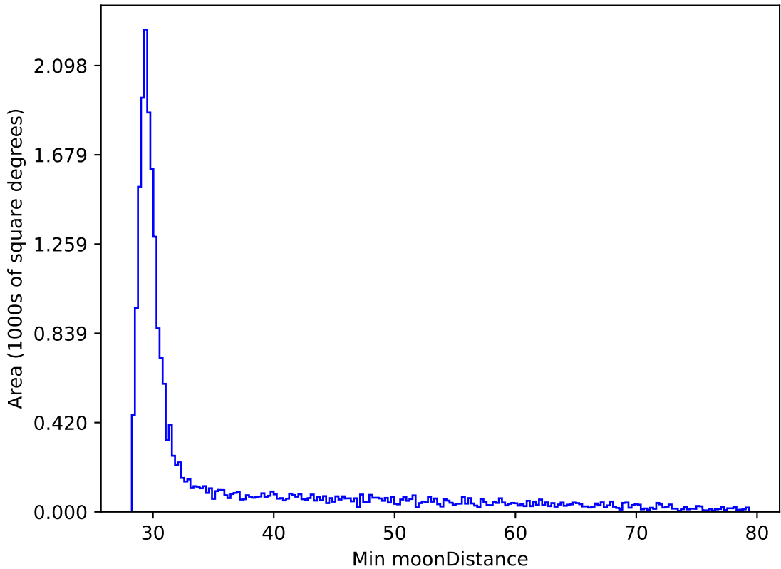
too_elab_r32_d3_giz_v3.4_10yrs All sky y band: Min moonDistance
