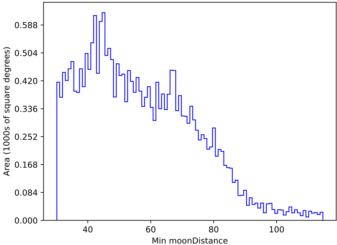
too_elab_r32_d3_giz_v3.4_10yrs All sky u band: Min moonDistance
