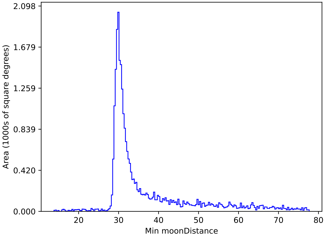
too_elab_r32_d3_giz_v3.4_10yrs All sky i band: Min moonDistance
