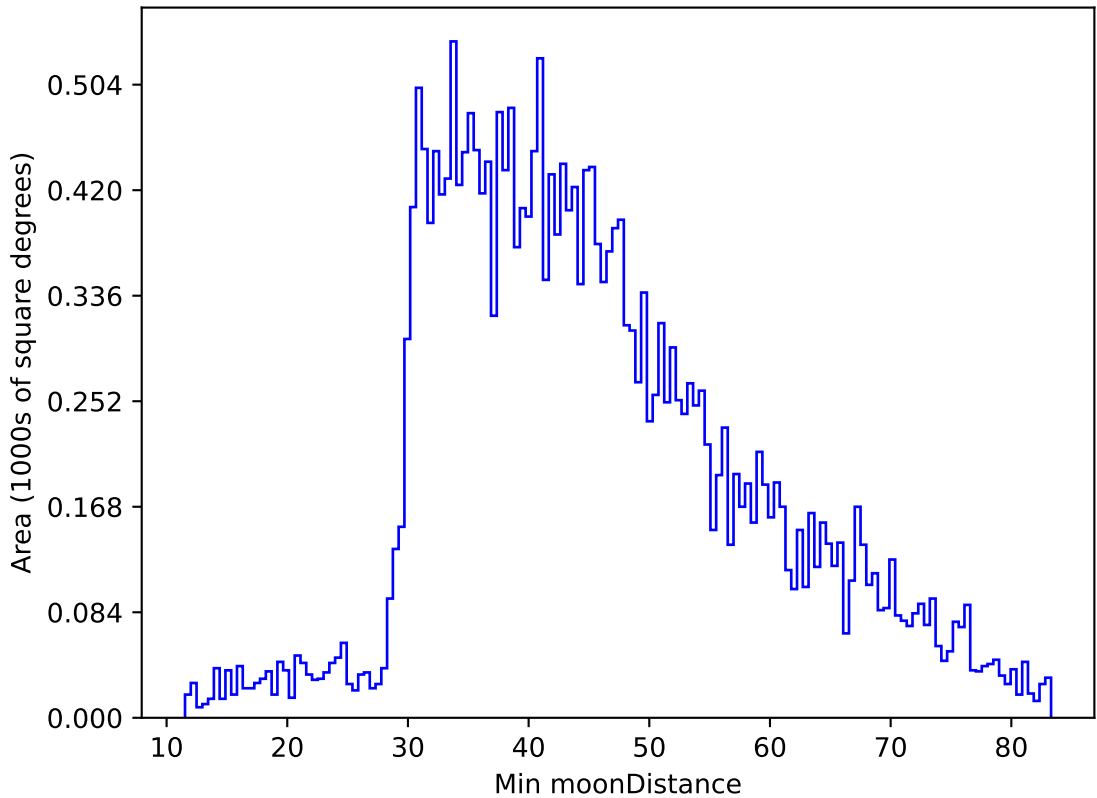
too_elab_r32_d3_giz_v3.4_10yrs All sky g band: Min moonDistance
