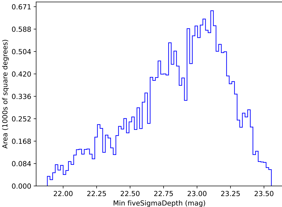
too_elab_r32_d3_giz_v3.4_10yrs Yr 1 u band: Min fiveSigmaDepth
