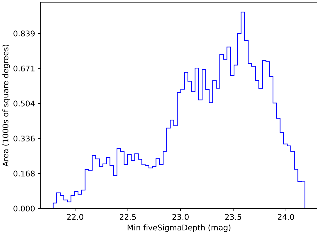
too_elab_r32_d3_giz_v3.4_10yrs Yr 1 r band: Min fiveSigmaDepth
