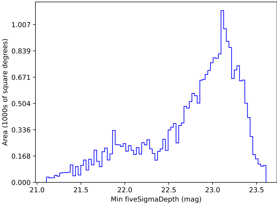
too_elab_r32_d3_giz_v3.4_10yrs Yr 1 i band: Min fiveSigmaDepth
