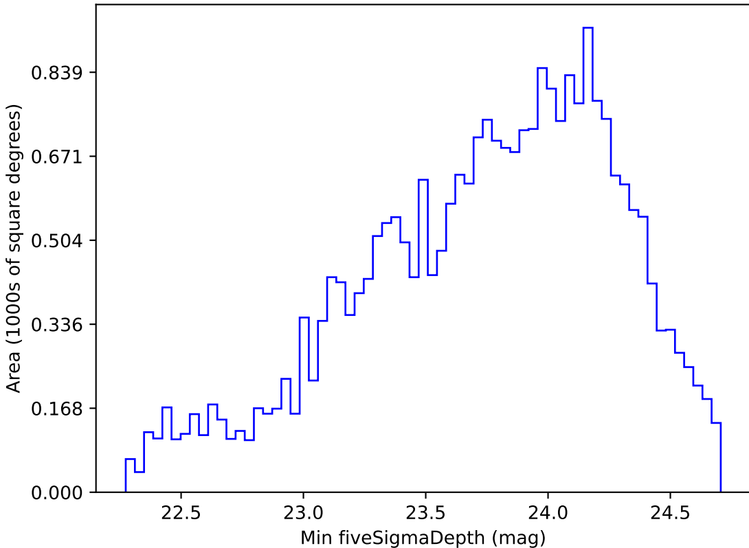
too_elab_r32_d3_giz_v3.4_10yrs Yr 1 g band: Min fiveSigmaDepth
