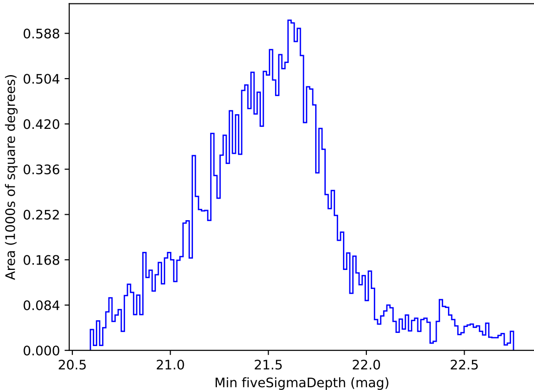
too_elab_r32_d3_giz_v3.4_10yrs Yr 1 all bands: Min fiveSigmaDepth
