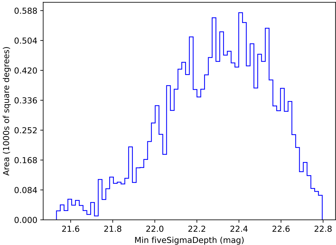
too_elab_r32_d3_giz_v3.4_10yrs WFD u band: Min fiveSigmaDepth
