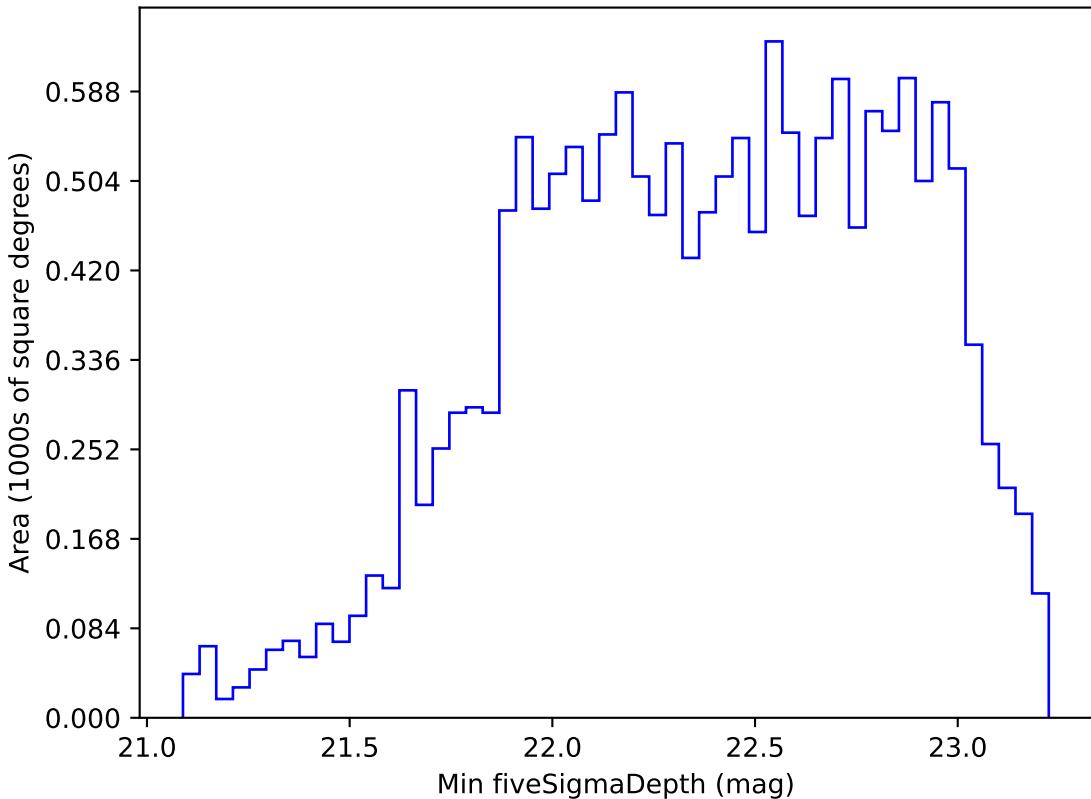
too_elab_r32_d3_giz_v3.4_10yrs WFD r band: Min fiveSigmaDepth
