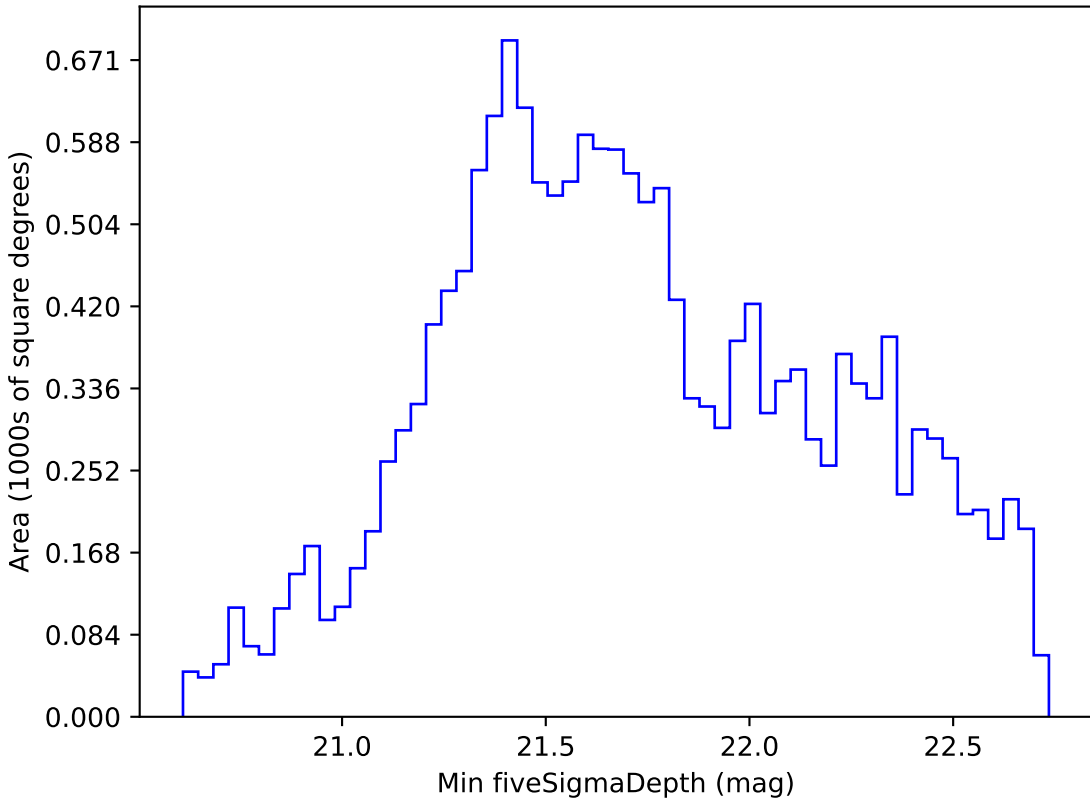
too_elab_r32_d3_giz_v3.4_10yrs WFD i band: Min fiveSigmaDepth
