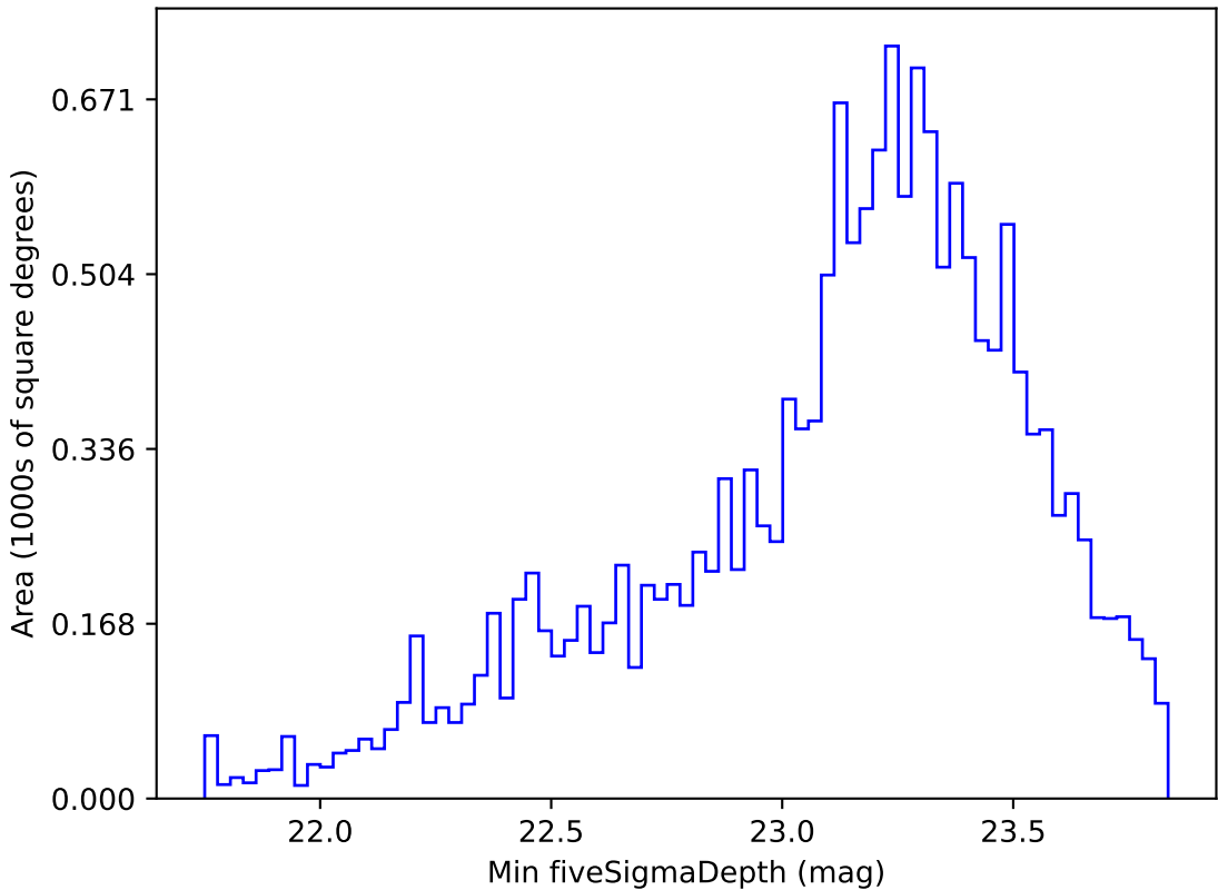
too_elab_r32_d3_giz_v3.4_10yrs WFD g band: Min fiveSigmaDepth
