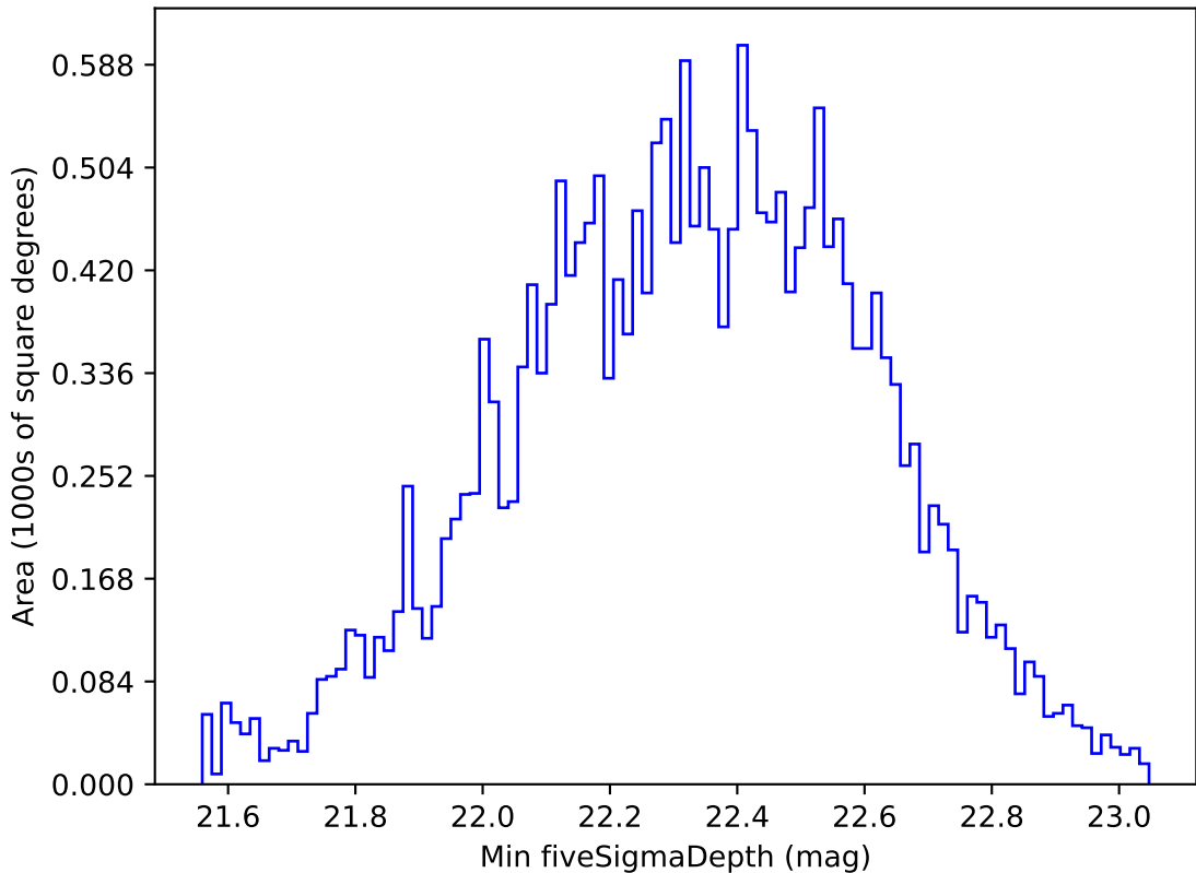
too_elab_r32_d3_giz_v3.4_10yrs All sky u band: Min fiveSigmaDepth
