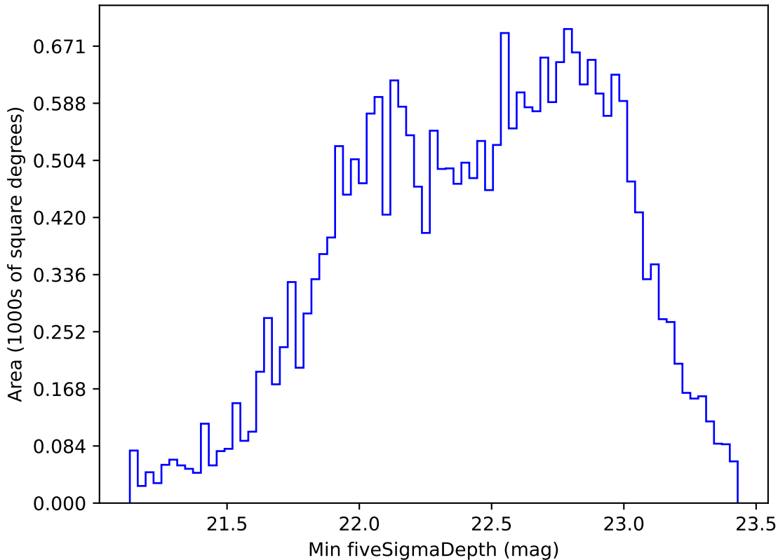
too_elab_r32_d3_giz_v3.4_10yrs All sky r band: Min fiveSigmaDepth
