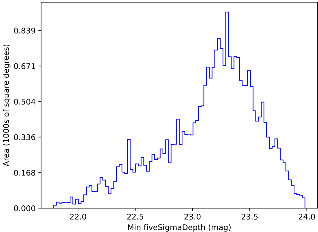
too_elab_r32_d3_giz_v3.4_10yrs All sky g band: Min fiveSigmaDepth
