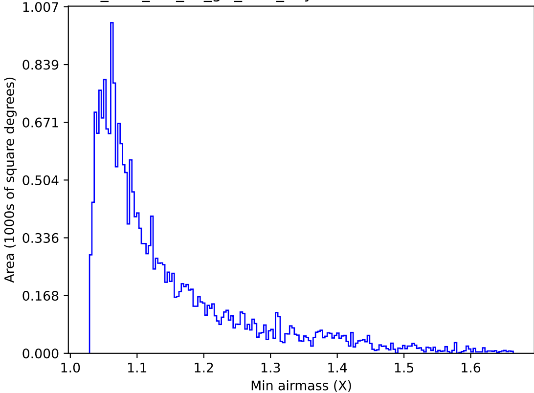
too_elab_r32_d3_giz_v3.4_10yrs Yr 1 u band: Min airmass
