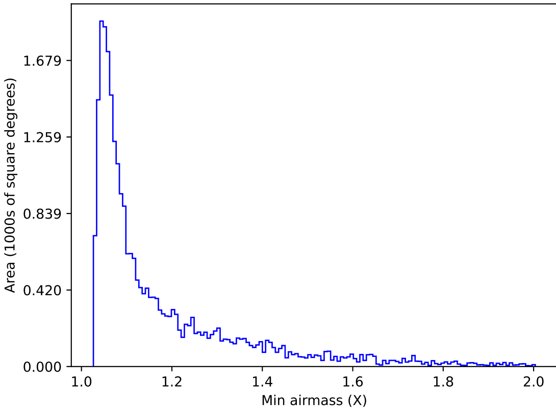
too_elab_r32_d3_giz_v3.4_10yrs Yr 1 g band: Min airmass
