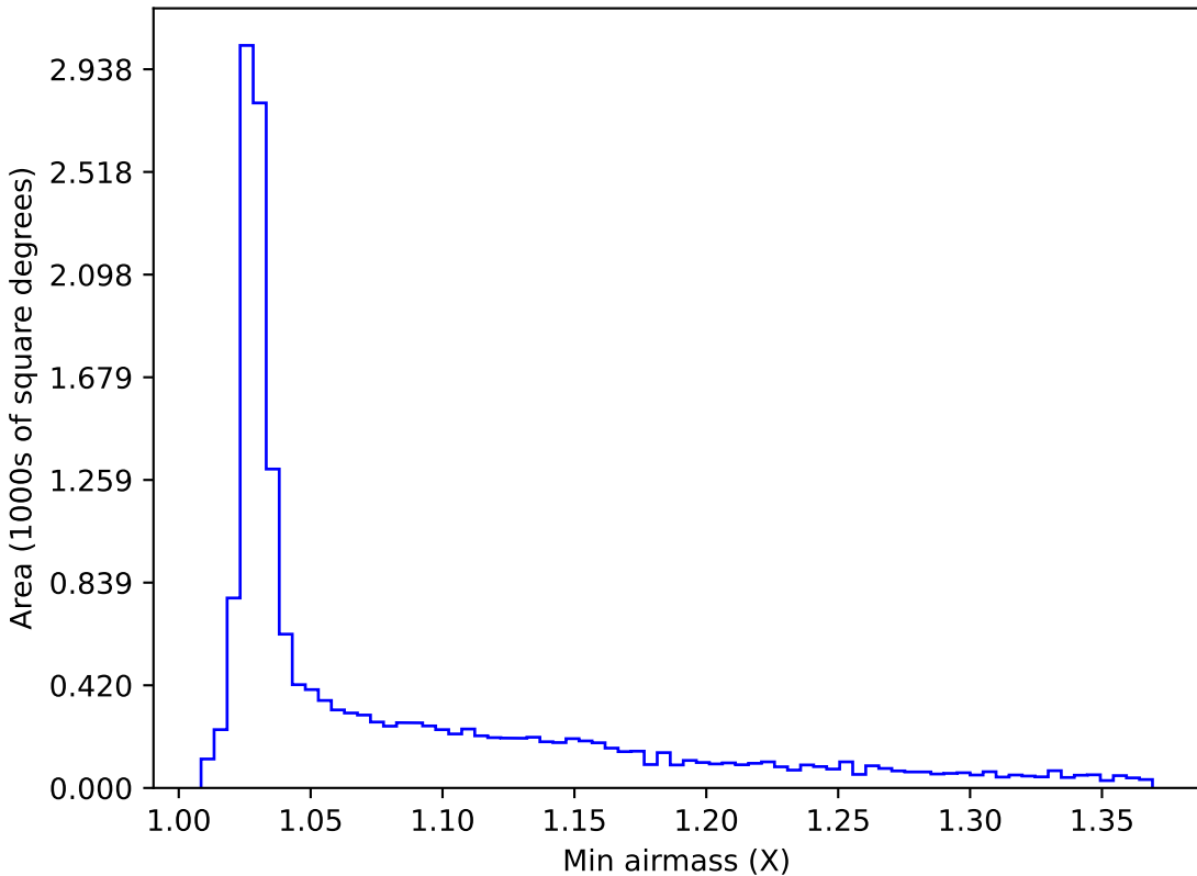
too_elab_r32_d3_giz_v3.4_10yrs WFD z band: Min airmass
