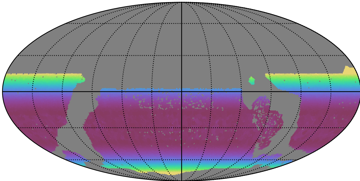
too_elab_r32_d3_giz_v3.4_10yrs WFD y band: Min airmass
