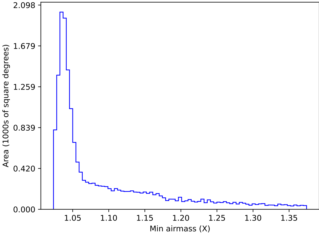
too_elab_r32_d3_giz_v3.4_10yrs WFD u band: Min airmass
