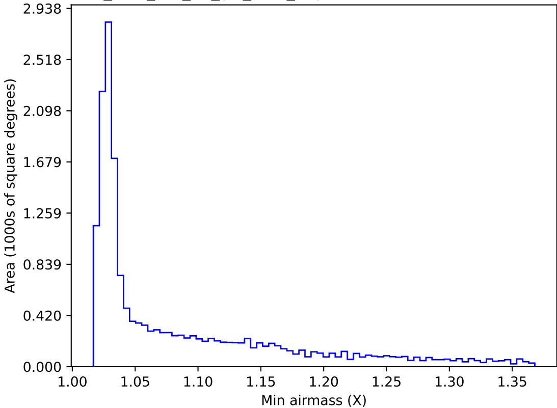
too_elab_r32_d3_giz_v3.4_10yrs WFD r band: Min airmass
