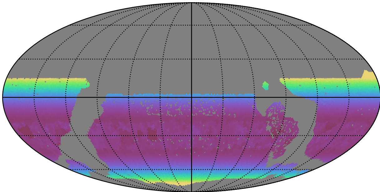
too_elab_r32_d3_giz_v3.4_10yrs WFD g band: Min airmass
