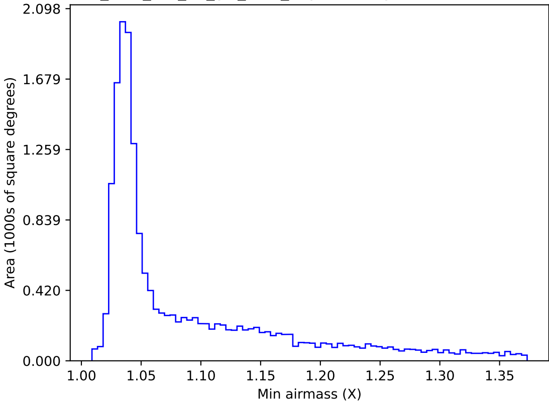
too_elab_r32_d3_giz_v3.4_10yrs WFD g band: Min airmass
