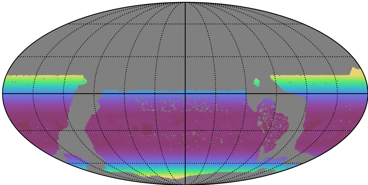
too_elab_r32_d3_giz_v3.4_10yrs WFD all bands: Min airmass
