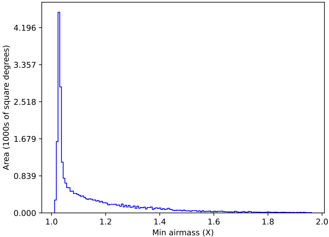
too_elab_r32_d3_giz_v3.4_10yrs All sky i band: Min airmass
