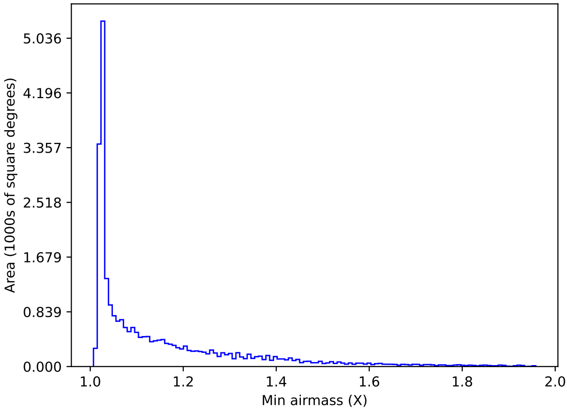
too_elab_r32_d3_giz_v3.4_10yrs All sky all bands: Min airmass
