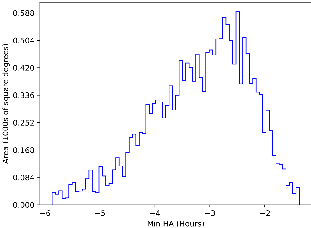
too_elab_r32_d3_giz_v3.4_10yrs WFD u band: Min HA
