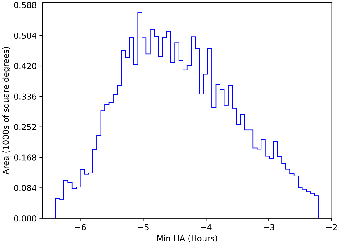
too_elab_r32_d3_giz_v3.4_10yrs WFD r band: Min HA
