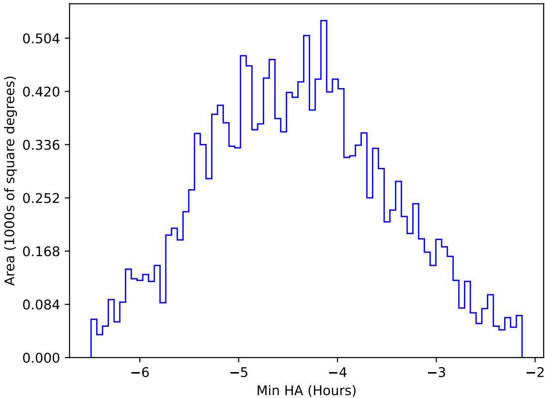
too_elab_r32_d3_giz_v3.4_10yrs WFD i band: Min HA
