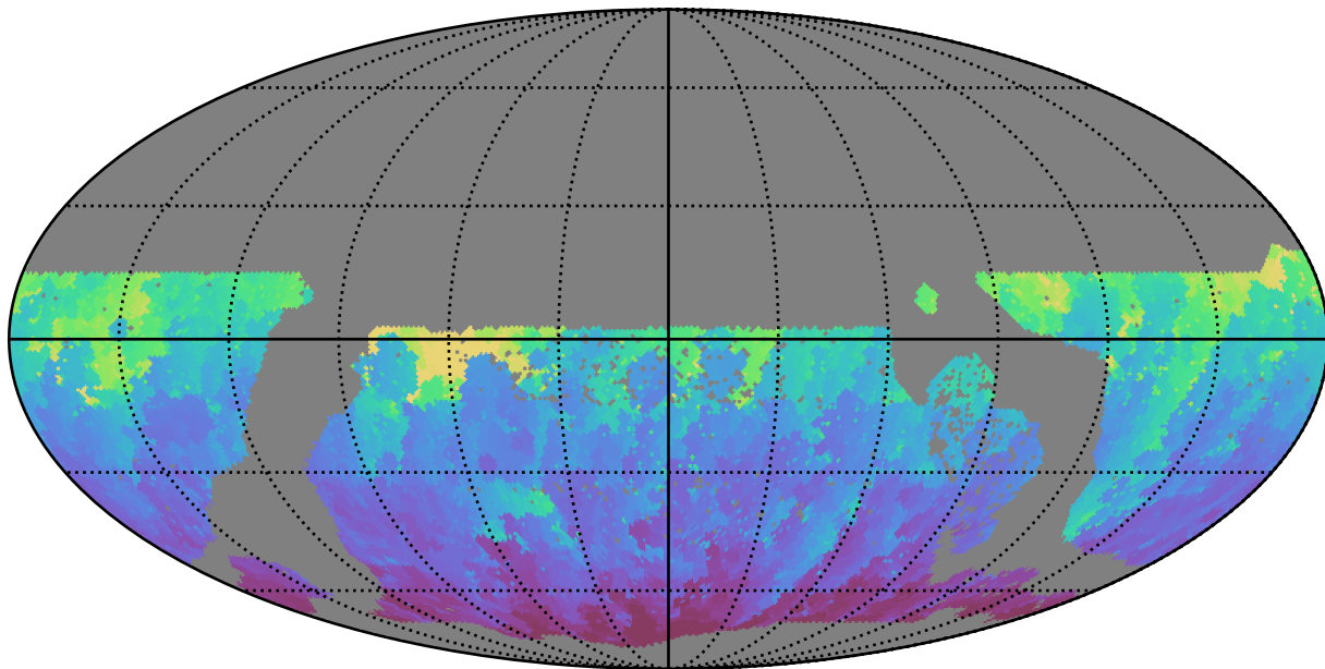
too_elab_r32_d3_giz_v3.4_10yrs WFD g band: Min HA
