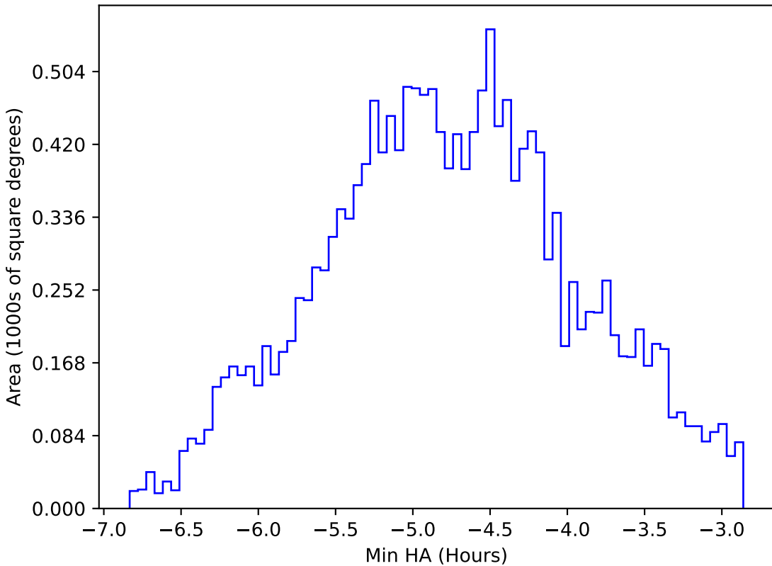
too_elab_r32_d3_giz_v3.4_10yrs WFD all bands: Min HA
