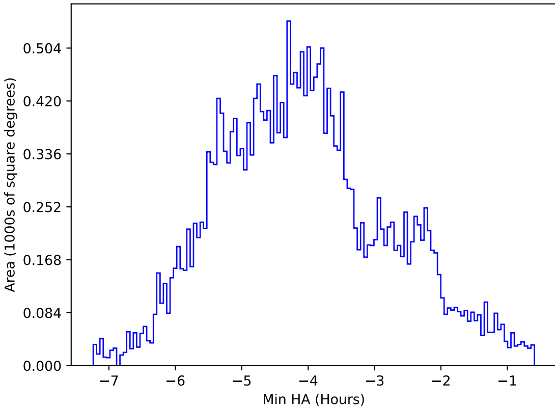
too_elab_r32_d3_giz_v3.4_10yrs All sky z band: Min HA
