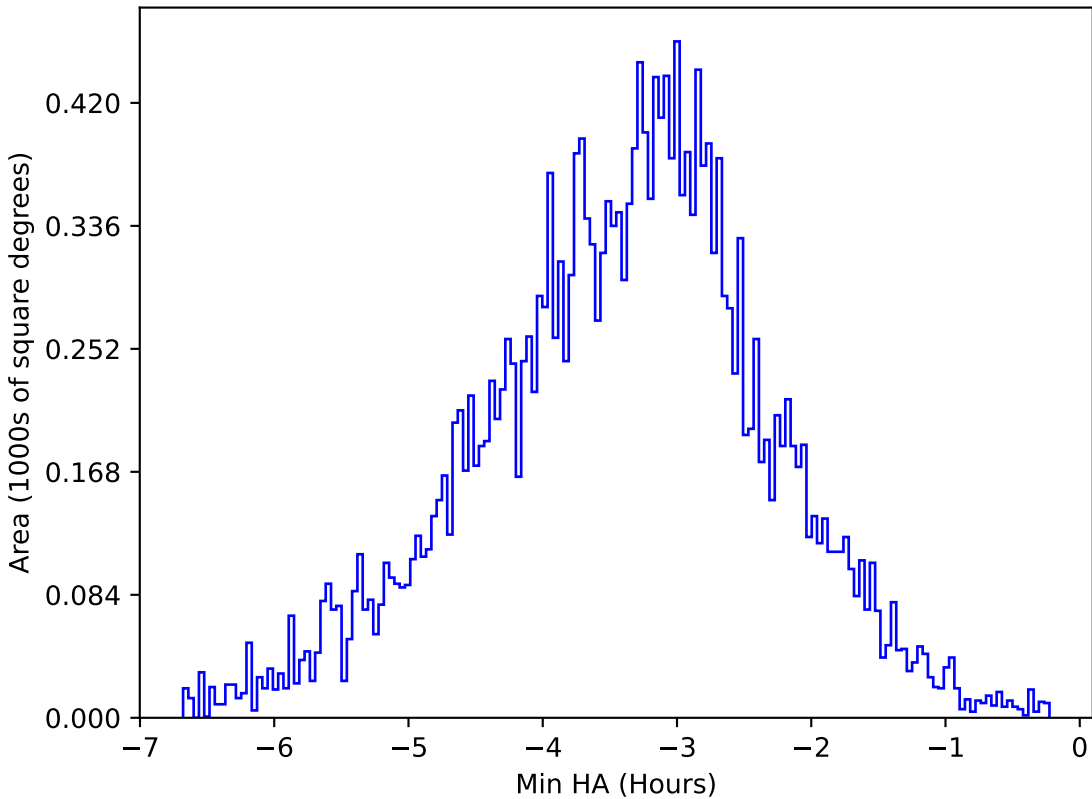
too_elab_r32_d3_giz_v3.4_10yrs All sky y band: Min HA
