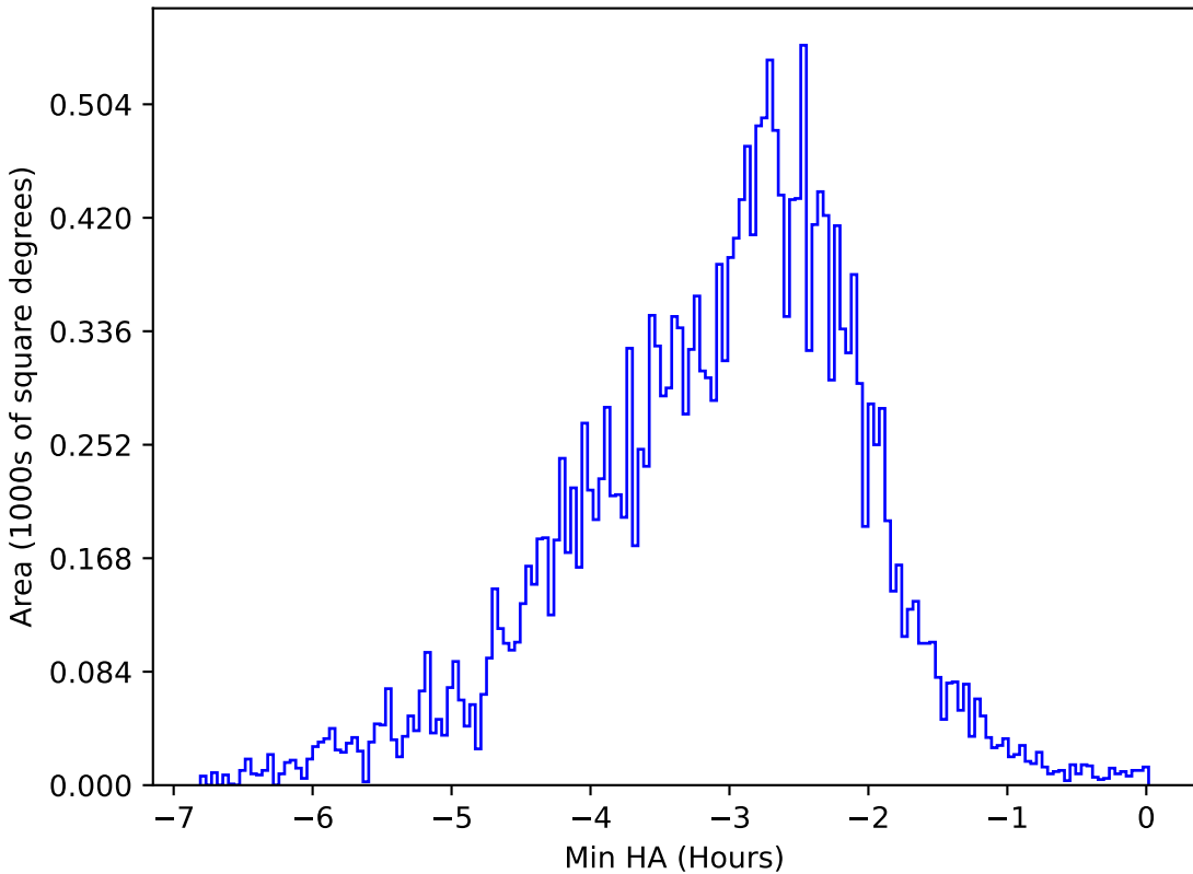
too_elab_r32_d3_giz_v3.4_10yrs All sky u band: Min HA
