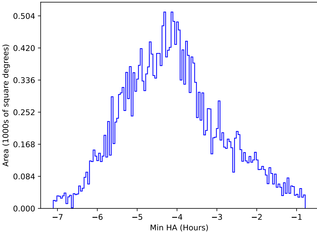
too_elab_r32_d3_giz_v3.4_10yrs All sky i band: Min HA
