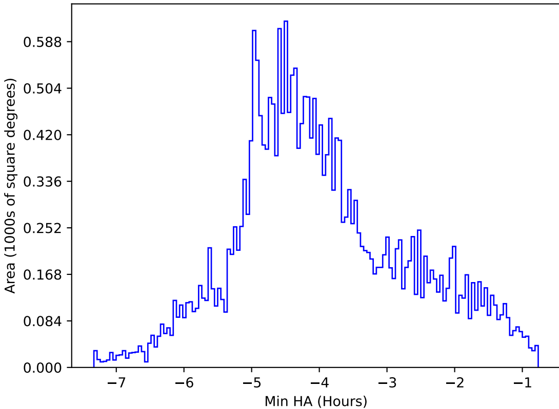
too_elab_r32_d3_giz_v3.4_10yrs All sky g band: Min HA
