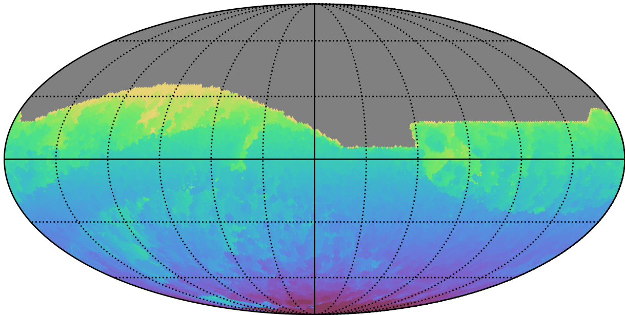
too_elab_r32_d3_giz_v3.4_10yrs All sky all bands: Min HA
