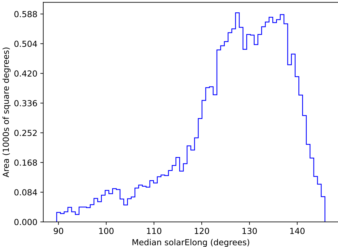
too_elab_r32_d3_giz_v3.4_10yrs WFD z band: Median solarElong
