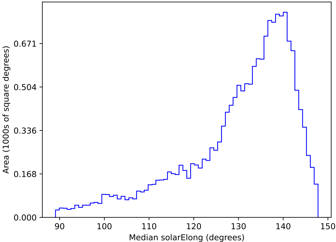
too_elab_r32_d3_giz_v3.4_10yrs WFD y band: Median solarElong
