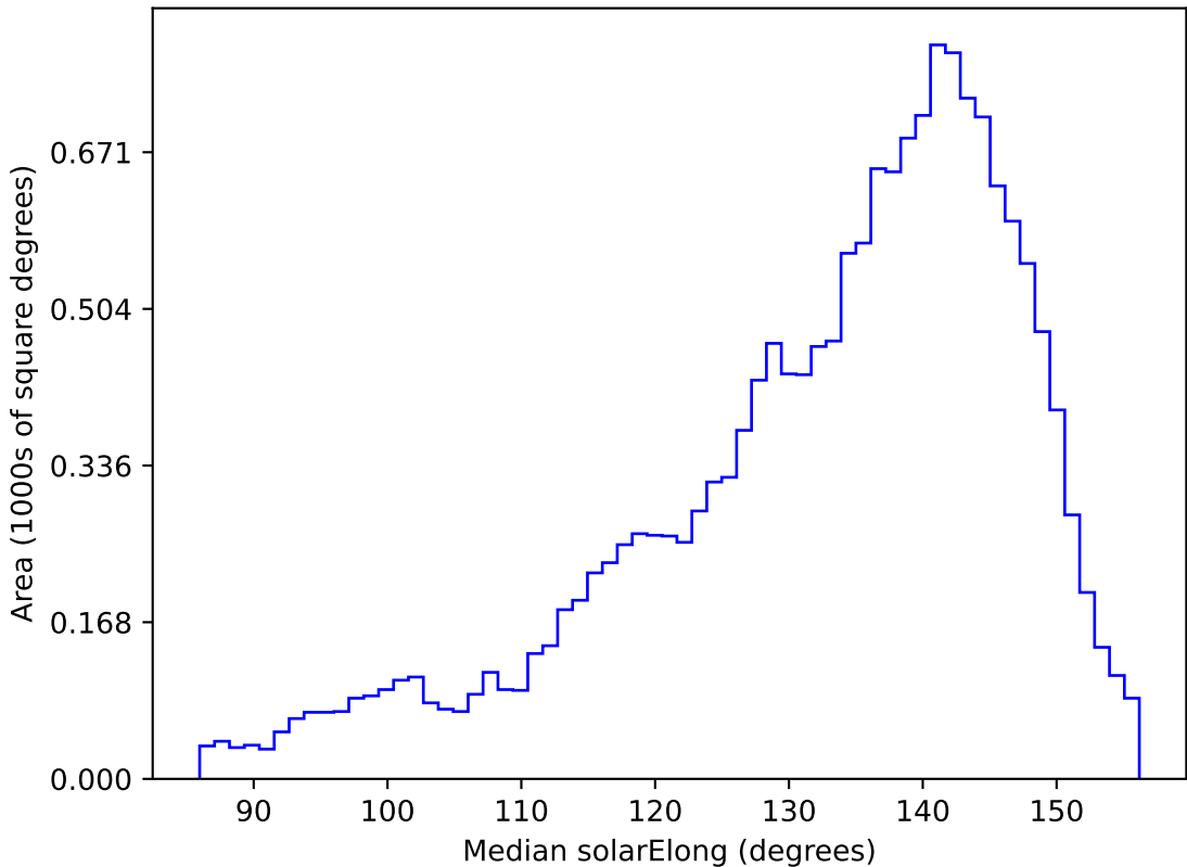
too_elab_r32_d3_giz_v3.4_10yrs WFD u band: Median solarElong
