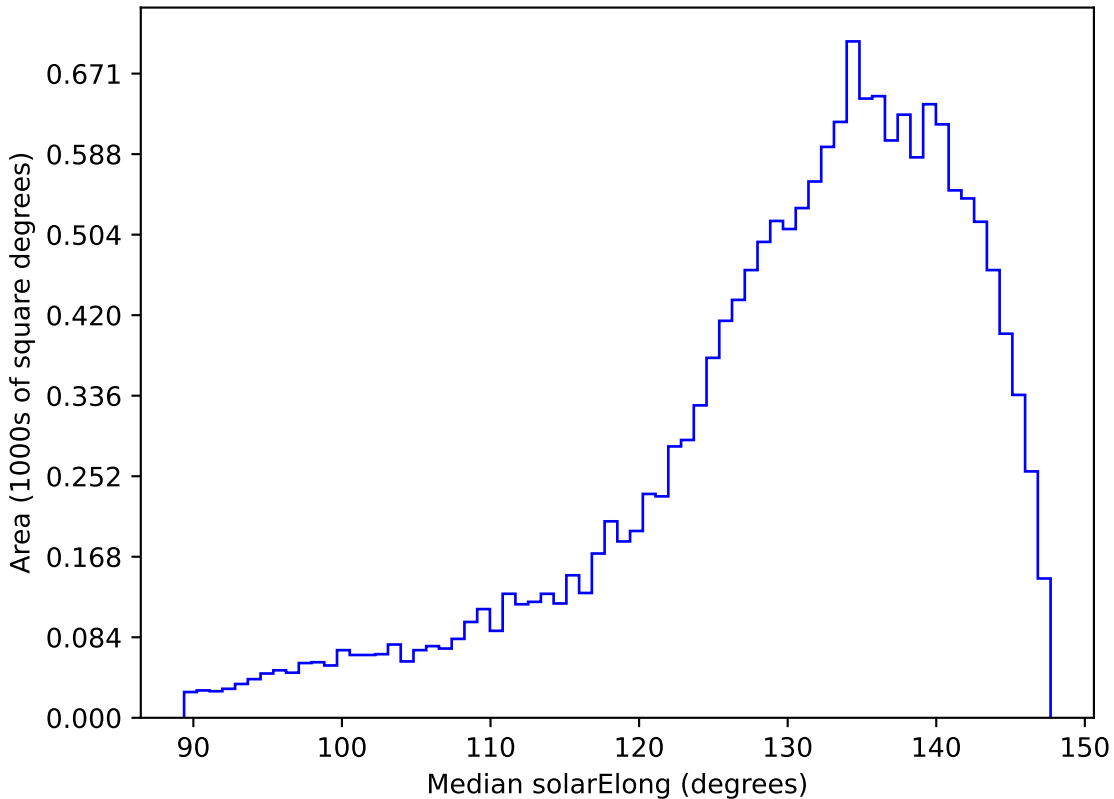
too_elab_r32_d3_giz_v3.4_10yrs WFD r band: Median solarElong
