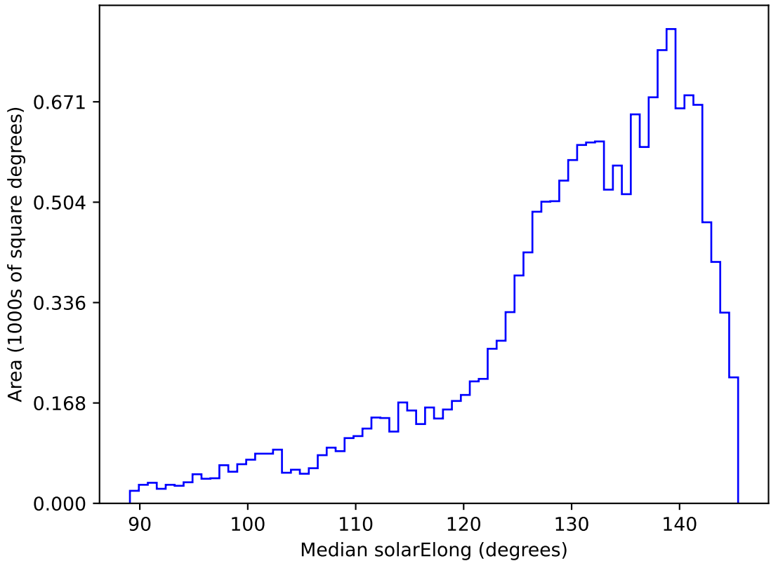
too_elab_r32_d3_giz_v3.4_10yrs WFD all bands: Median solarElong
