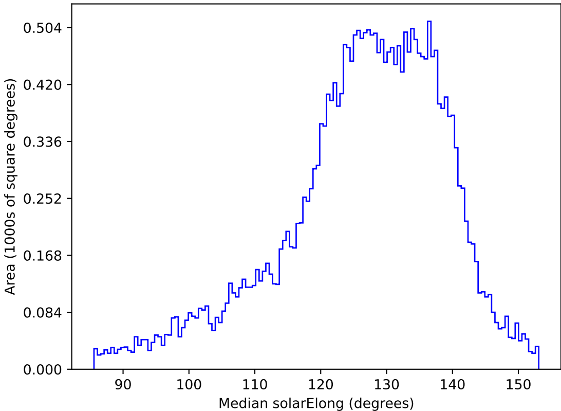
too_elab_r32_d3_giz_v3.4_10yrs All sky z band: Median solarElong
