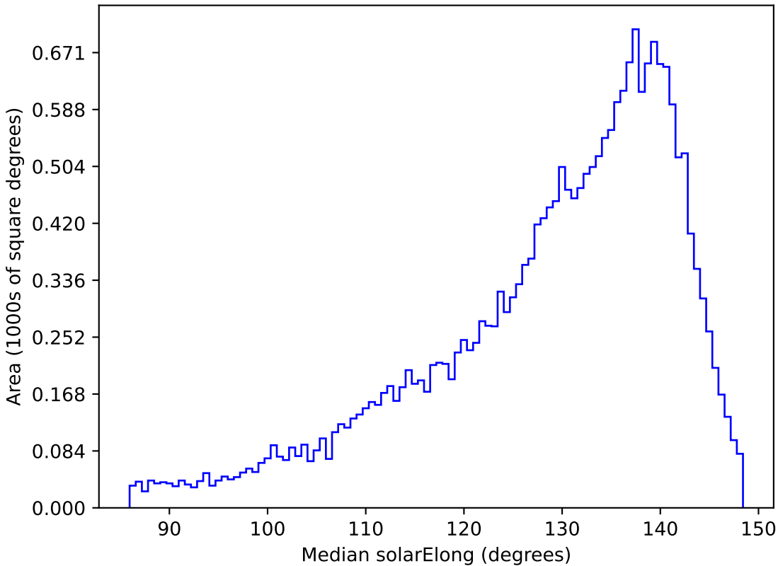
too_elab_r32_d3_giz_v3.4_10yrs All sky y band: Median solarElong
