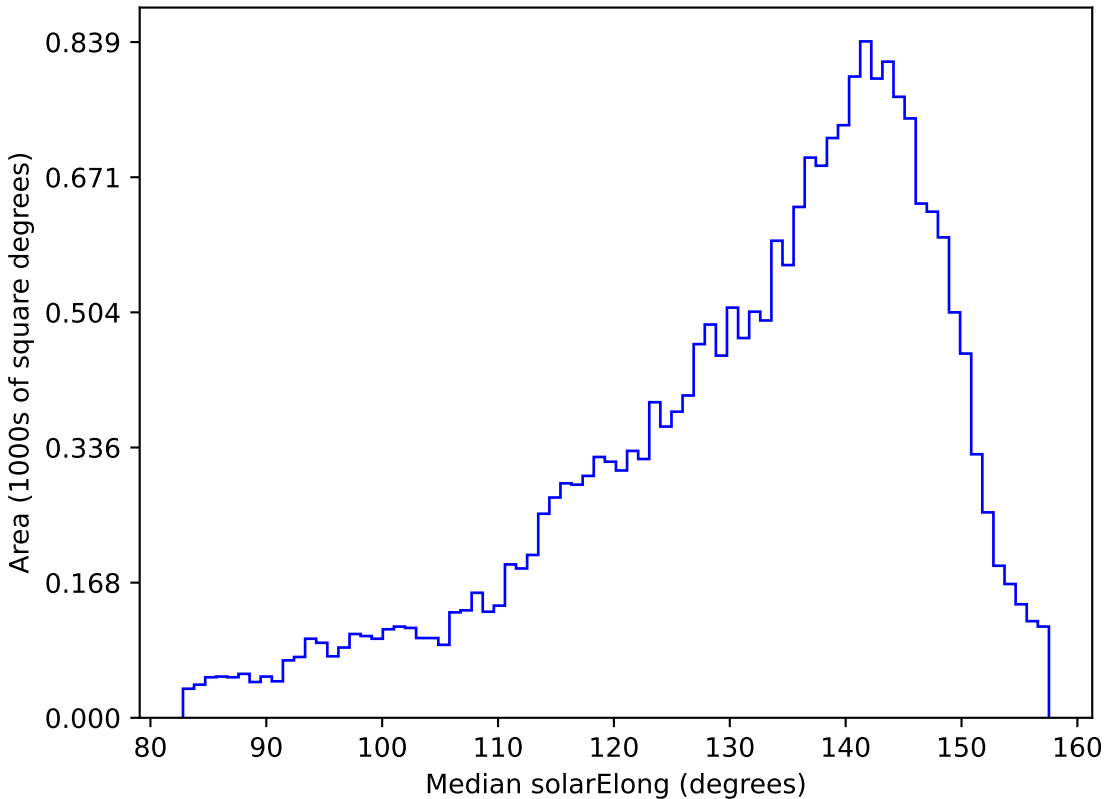
too_elab_r32_d3_giz_v3.4_10yrs All sky u band: Median solarElong
