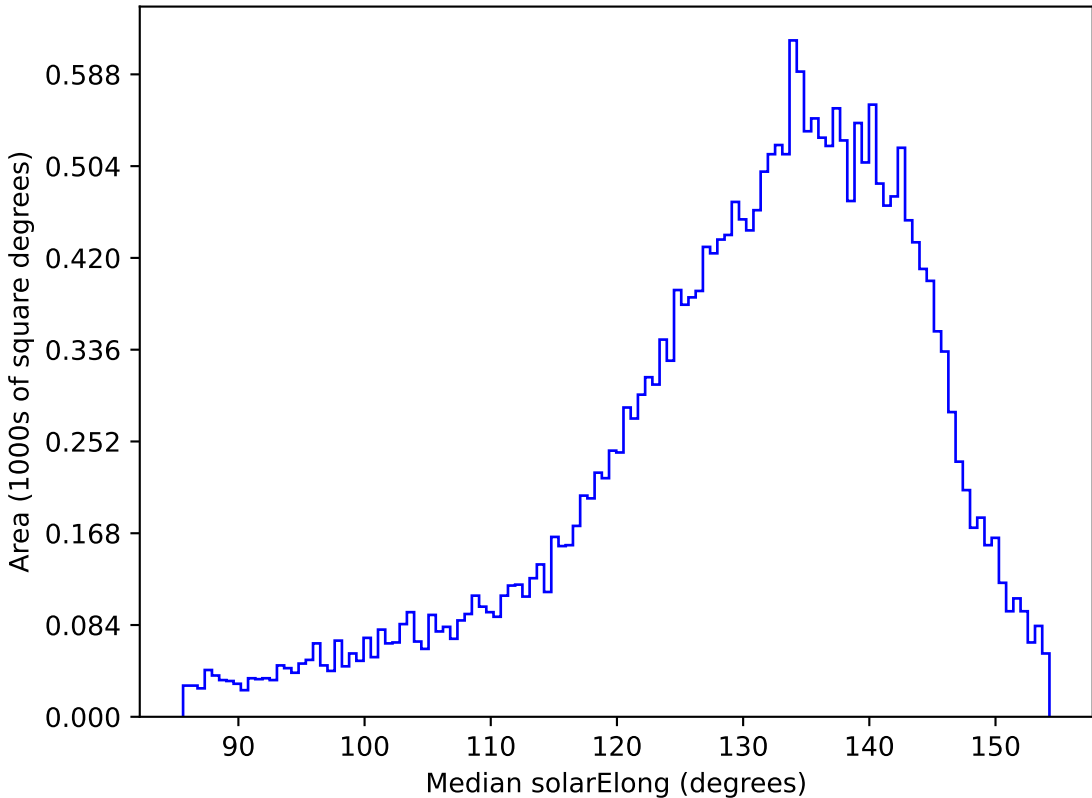
too_elab_r32_d3_giz_v3.4_10yrs All sky r band: Median solarElong
