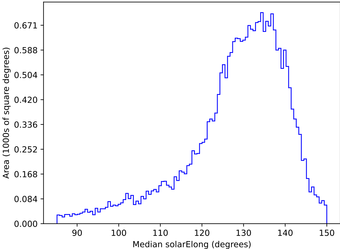
too_elab_r32_d3_giz_v3.4_10yrs All sky i band: Median solarElong
