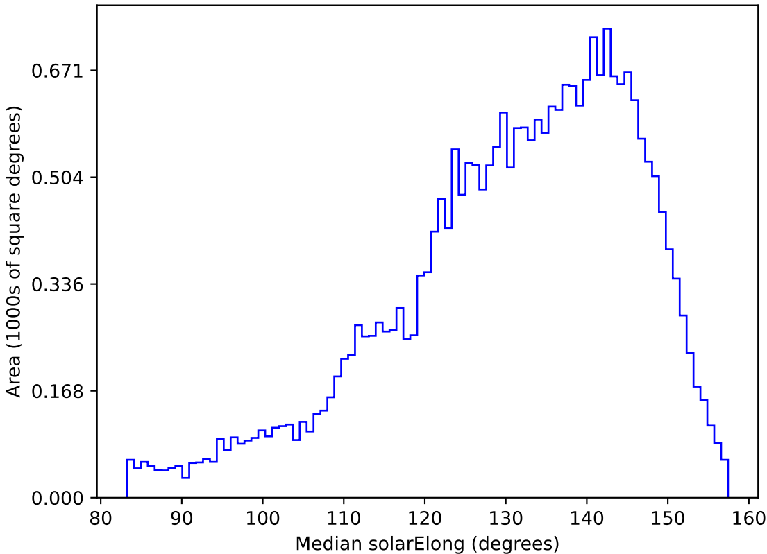
too_elab_r32_d3_giz_v3.4_10yrs All sky g band: Median solarElong
