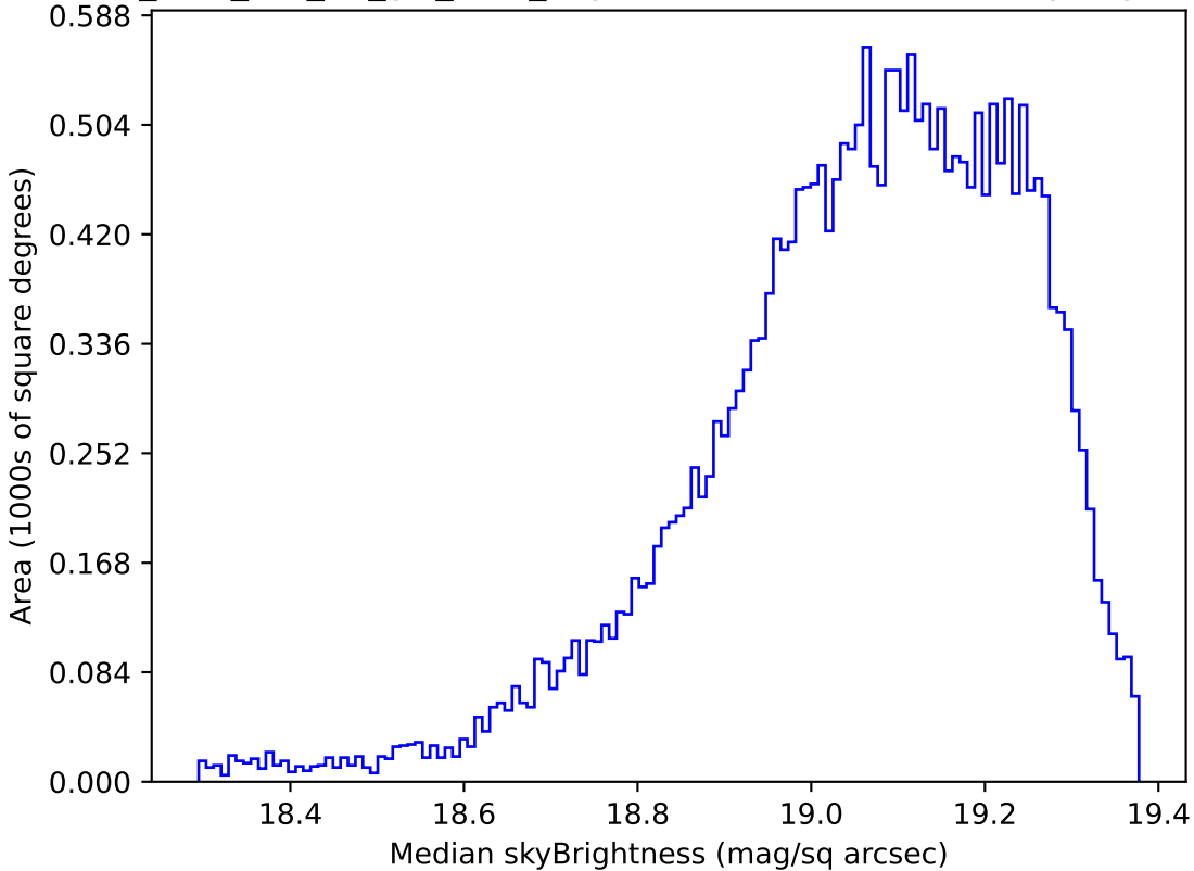
too_elab_r32_d3_giz_v3.4_10yrs Yr 1 z band: Median skyBrightness
